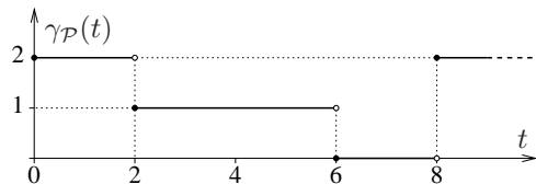
Figure 3. Example of characteristic function \gamma_{\mathcal{P}} .
