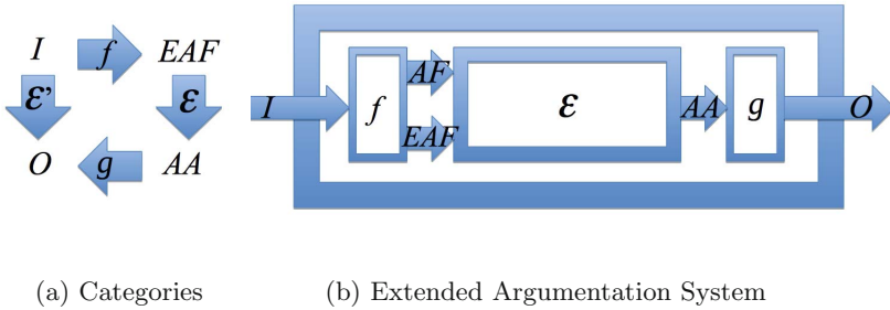
Figure 5. Extending Dung’s theory: a function f transforms an argumentation input I to an extended argumentation framework EAF , which contains besides attack relations among arguments represented in AF also other kind of relations among arguments. As in Figure 4, the argumentation output is a function of the argumentation input O = \mathcal{E}'(I) , derived from the two transformations and the acceptance function, O = \mathcal{E}'(I) = g(AA) = g(\mathcal{E}(EAF)) = g(\mathcal{E}(f(I))) .
