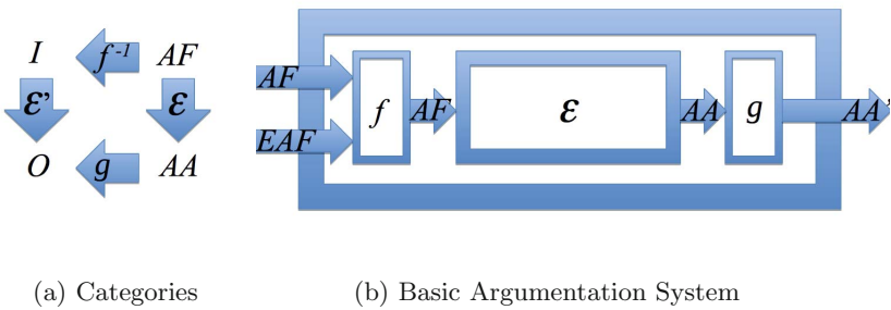
Figure 8. The methodological problem: how to use Dung’s acceptance functions \mathcal{E} to find functions \mathcal{E}' between argumentation input I and argumentation output O ? This function transformation consists of two parts: a function f^{-1} transforms an argumentation framework AF to an argumentation input I , and a function g transforms the accepted arguments into argumentation output. Summarizing \mathcal{E}' = \{(f^{-1}(a), g(b)) \mid (a, b) \in \mathcal{E}\} .
