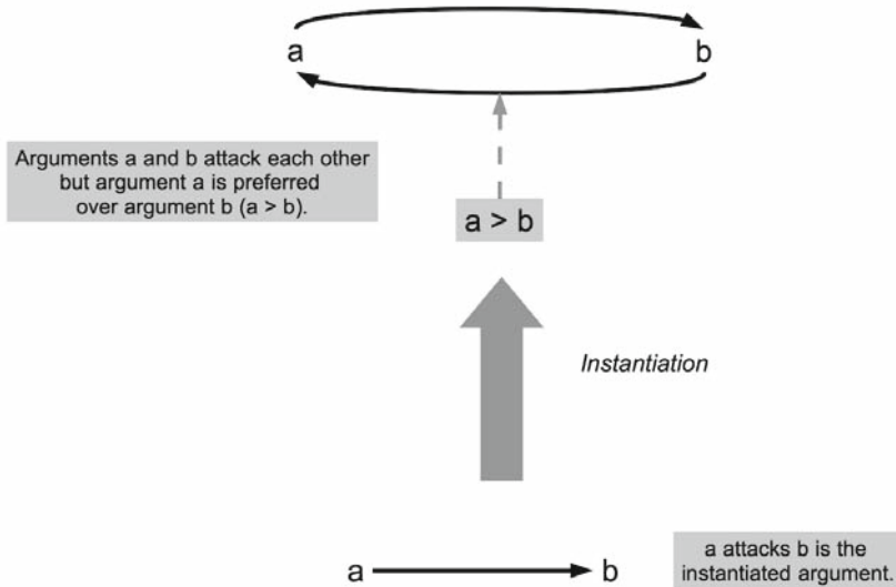
Figure 3. Instantiation of an abstract argument.
