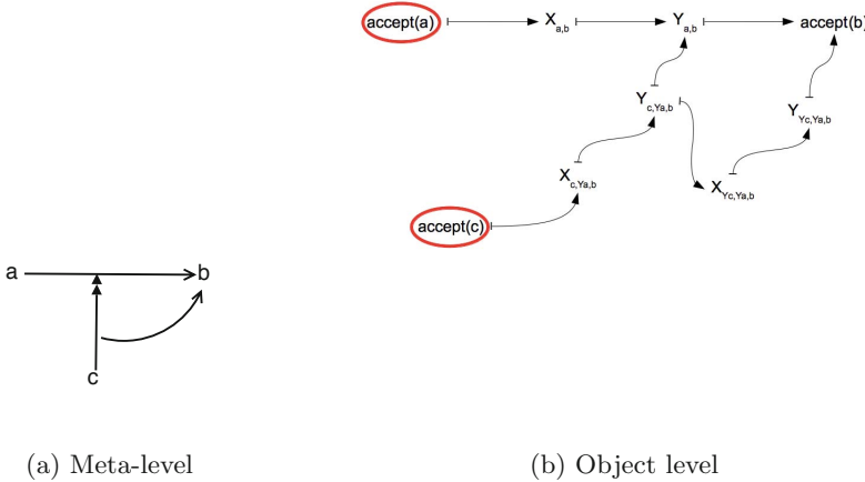
Figure 17. An argumentation network in the meta level (a) and object level (b).
