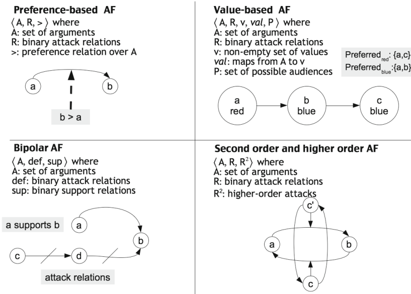
Figure 11. Examples of extended argumentation frameworks.
