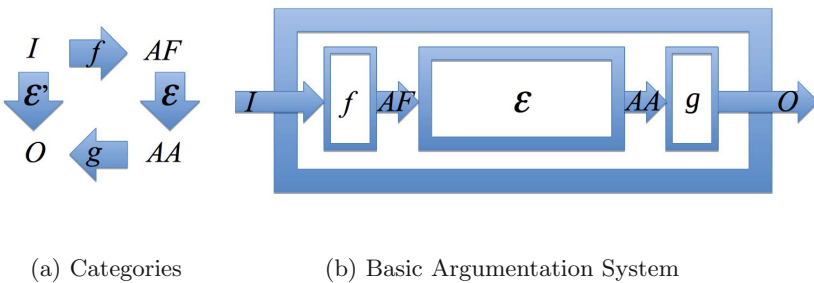
Figure 4. Instantiating Dung’s basic argumentation theory: a function f transforms an argumentation input I to an argumentation framework AF , whose extensions of accepted arguments AA = \mathcal{E}(AF) are transformed back into the argumentation output O = \mathcal{E}'(I) , derived from the two transformations and the acceptance function. Summarizing O = \mathcal{E}'(I) = g(AA) = g(\mathcal{E}(AF)) = g(\mathcal{E}(f(I))) .
