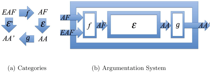
Figure 6. Extended argumentation framework as an instantiation: a function f transforms an extended argumentation framework EAF to a basic argumentation framework AF . As in Figure 4, the accepted arguments of the extended framework are a function of the extended argumentation framework AA = \mathcal{E}'(EAF) , derived from the two transformations and the acceptance function of basic argumentation, AA' = \mathcal{E}'(EAF) = g(AA) = g(\mathcal{E}(AF)) = g(\mathcal{E}(f(EAF))) .
