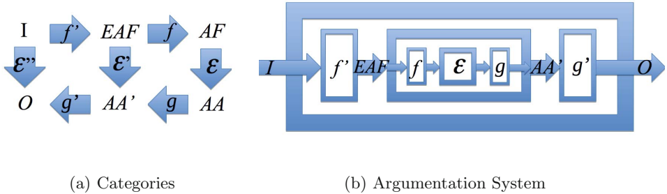
Figure 7. Combining instantiation and extended argumentation frameworks: a function f' transforms an argumentation input I to an extended argumentation framework EAF , and a function f translates this extended argumentation framework to a basic argumentation framework AF . As in Figure 4, the argumentation output is a function of the argumentation input O = \mathcal{E}''(I) , derived from the two transformations f' and g' , and the acceptance function \mathcal{E}' . Moreover, as in Figure 6, the acceptable arguments of the extended argumentation framework are a function of the extended argumentation function AA' = \mathcal{E}'(EAF) , derived from the two transformations f and g , and the acceptance function \mathcal{E} . Summarizing O = \mathcal{E}''(I) = g'(AA') = g'(\mathcal{E}'(EAF)) = g'(\mathcal{E}'(f'(I))) = g'(g(\mathcal{E}(f(f'(I)))) .
