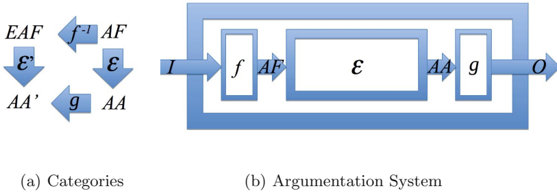
Figure 9. The meta-argumentation methodology: we use Dung’s acceptance functions \mathcal{E} to find functions \mathcal{E}' between extended argumentation frameworks EAF and acceptable arguments AA' . This function transformation consists of two parts: a function f^{-1} transforms an argumentation framework AF to an extended argumentation framework EAF , and a function g transforms the accepted arguments of the basic argumentation framework into acceptable arguments of the extended argumentation frameworks. Summarizing \mathcal{E}' = \{(f^{-1}(a), g(b)) \mid (a, b) \in \mathcal{E}\} .
