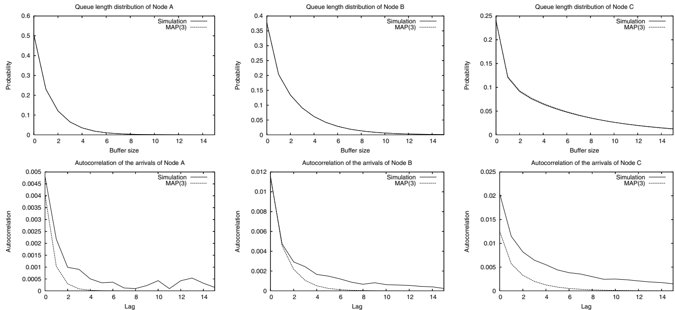
Fig. 6. Autocorrelation of arrivals and queue length distribution of nodes in Example 3
