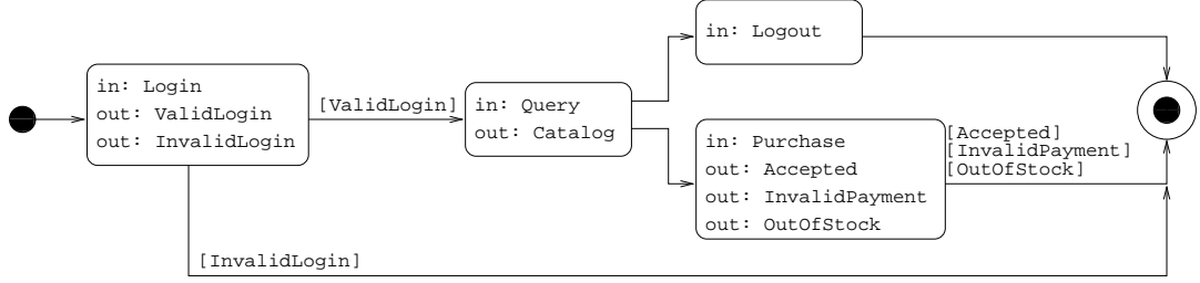
Figure 1. Contract of a simple e-commerce service as a WSCL diagram.
