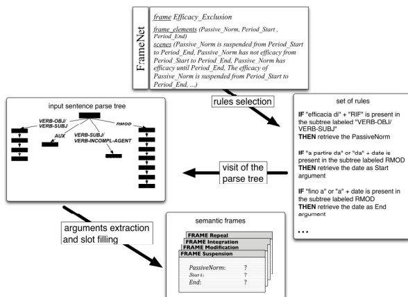
Figure 2 – The semantic interpretation process.
