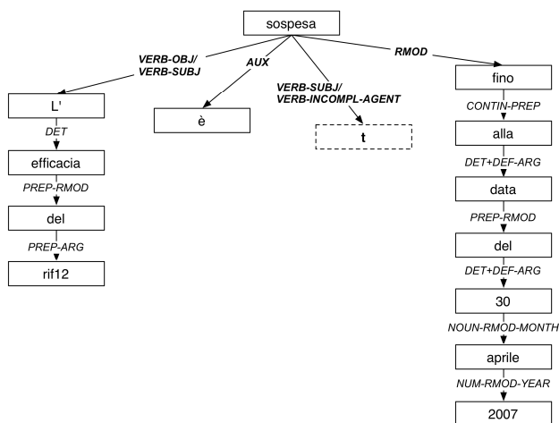
Figure 1 – The (simplified) dependency tree structure for sentence “The efficacy of the rif12 is suspended until the date of April 30th, 2007”.
