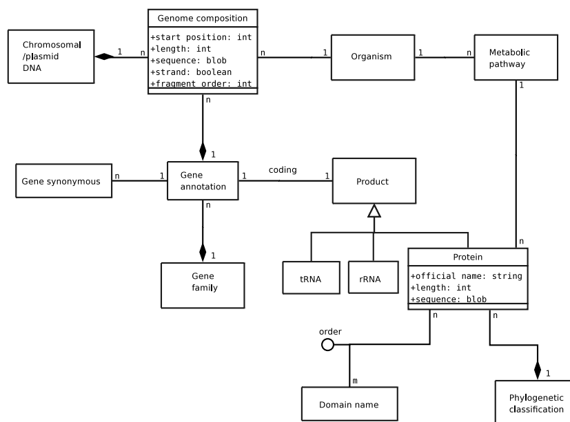
Fig. 1. Star schema of BIOBITS Data Mart
