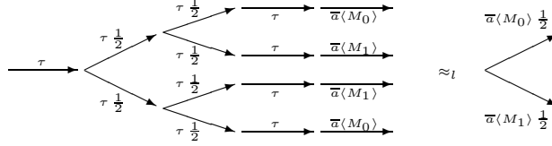
Fig. 1. \nu c.\text{OT}_2^1(S, R, M_0, M_1) \approx_l \bar{a}\langle M_0 \rangle \oplus_{\frac{1}{2}} \bar{a}\langle M_1 \rangle .
