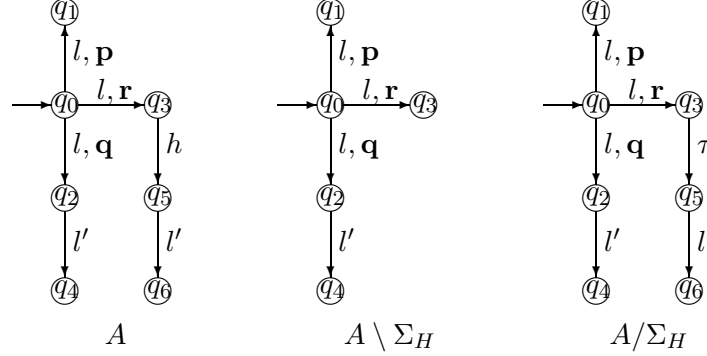
Figure 1. A probabilistic covert channel.
