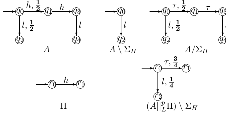
Figure 3. A \in PTNI , but A \notin PTNDC .
