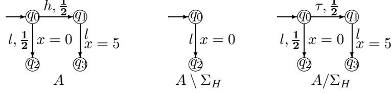
Figure 2. A timing covert channel.
