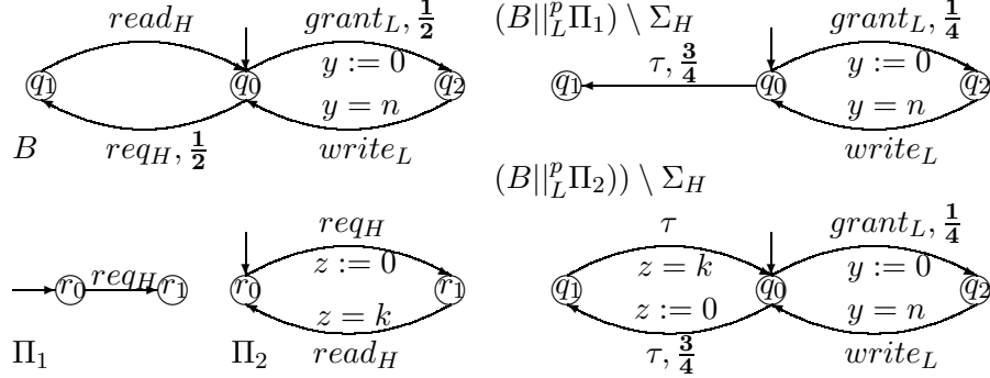
Figure 4. Device specification with timing covert channels.
