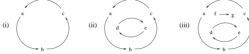
Fig. 1. (i) represents (a \cdot b \cdot c)^L ; (ii) represents (a \cdot b \cdot c)^L \upharpoonright (d \cdot e)^L ; (iii) represents (a \cdot b \cdot c)^L \upharpoonright ((d \cdot e)^L \upharpoonright f \cdot g) .
