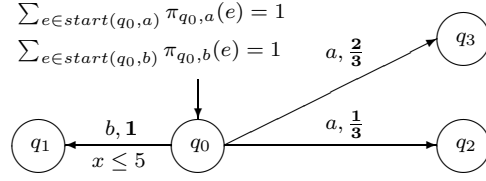
Fig. 1. Example of Probabilistic Timed Automaton
